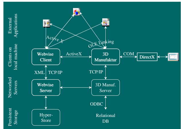
Figure 4: Integration architecture of Manufaktur
