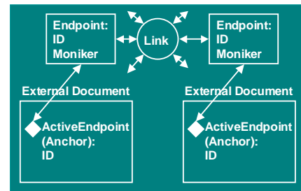
Figure 5: ActiveEndpoints
