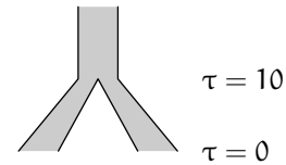
Figure 3: Two populations merging at time \tau = 10 .
