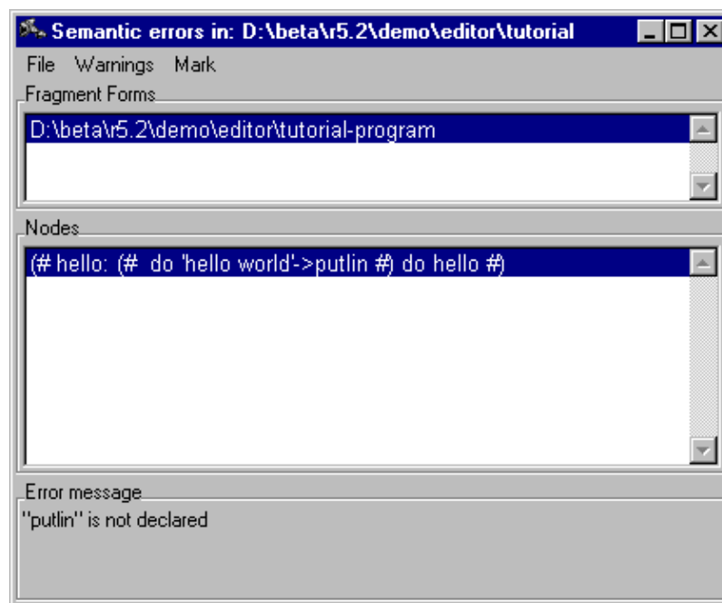
Figure 6: Semantic Errors Viewer
